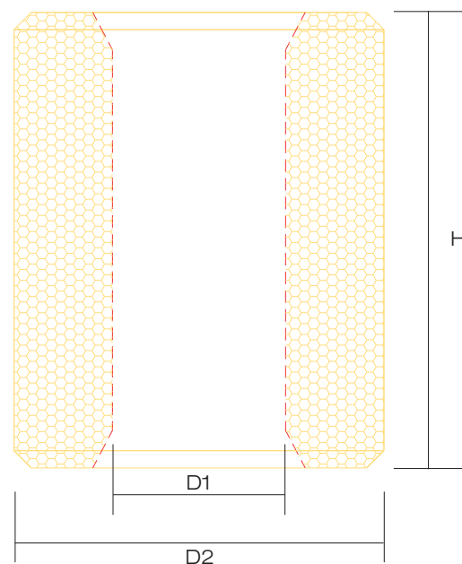
SOLID CORE
