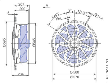
Design H - ZApplus Flattop, guard grille pressure side
