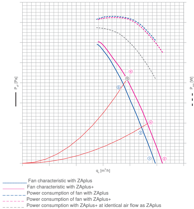
Increase in air flow rate ZAplus+ vs ZAplus
